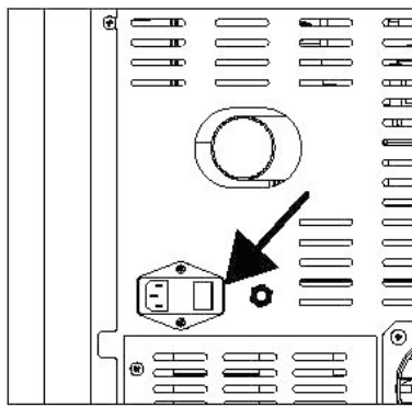
fig. 14 electric connection of the boiler
