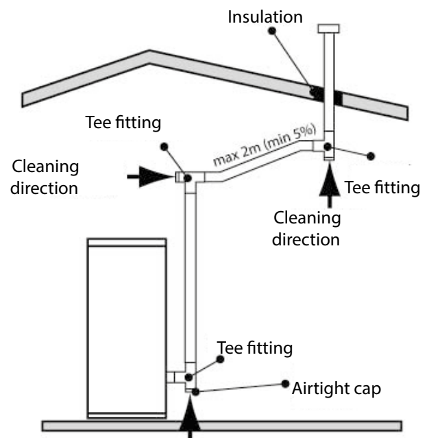
fig. 11 pipe length
