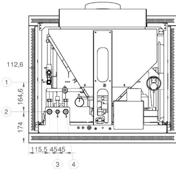
fig. 10 connection points without a DHW kit
