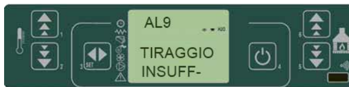
fig. 44 control panel - insufficient draught
