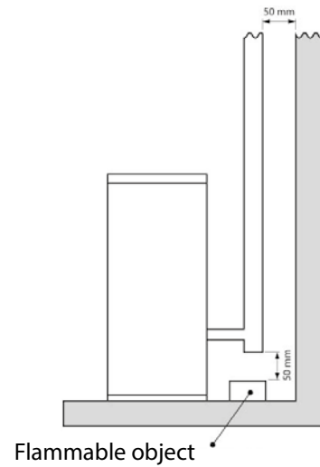
fig. 6 minimum safety clearances for positioning product
