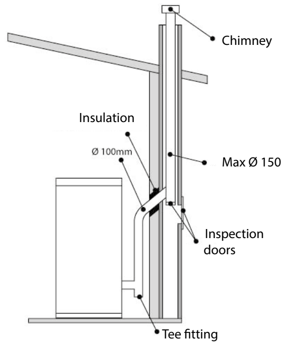
fig. 9 traditional flue
