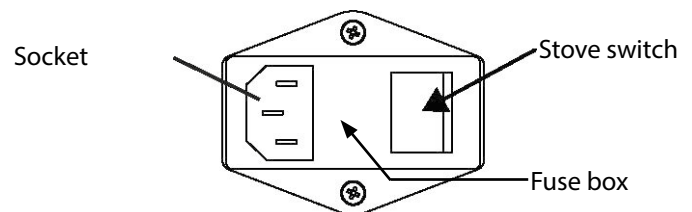
fig. 12 electric power supply
