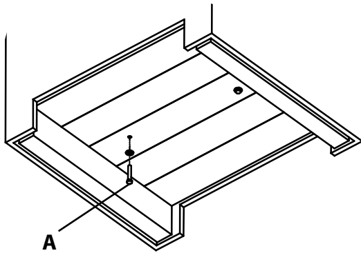
fig. 3 fixing removal
