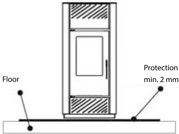
fig. 7 floor protections
