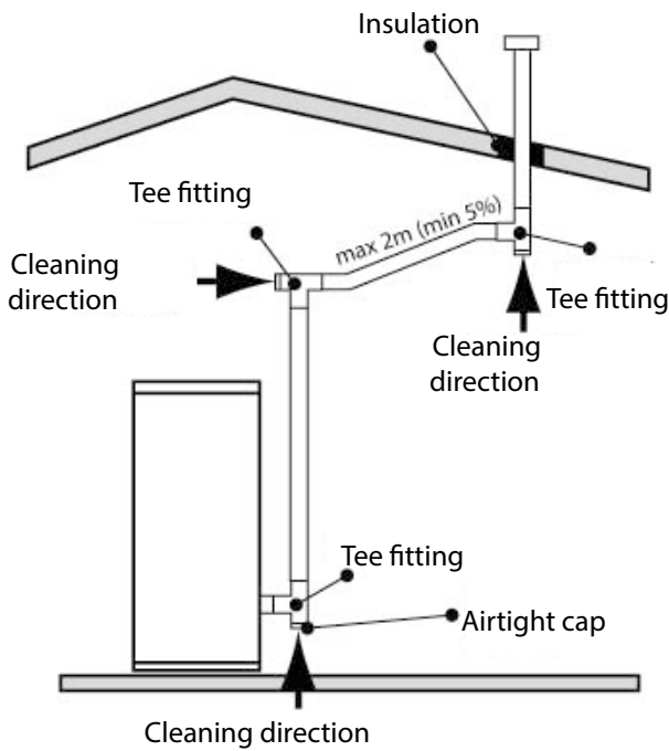
fig. 8 pipe length
