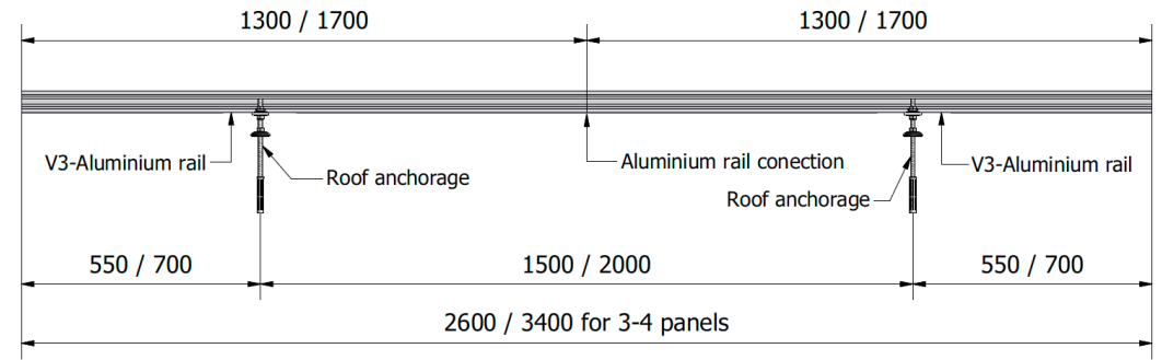
Support structure - Photovoltaic module (Front view)
