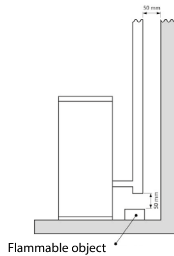
fig. 6 minimum safety clearances for positioning product
