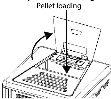
fig. 13 pellet loading
